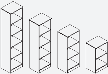
FS100 FS100-83: W 45 x D 36.6 x H 83 FS100-120.5: W 45 x D 36.6 x H 120.5 FS100-158: W 45 x D 36.6 x H 158 FS100-195.5: W 45 x D 36.6 x H 195.5
