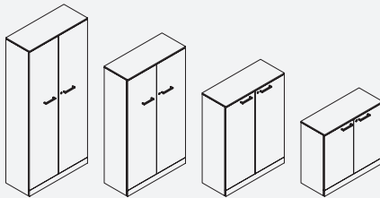
FS250 FS250-83: W 90 x D 36.6 x H 83 FS250-120.5: W 90 x D 36.6 x H 120.5 FS250-158: W 90 x D 36.6 x H 158 FS250-195.5: W 90 x D 36.6 x H 195.5 Capability of ordering mangnetic door
