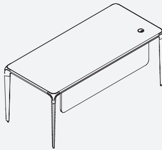
CD500 CD500-120: W 120 x D 75 x H 76 CD500-140: W 140 x D 75 x H 76 CD500-160: W 160 x D 75 x H 76 CD500-180: W 180 x D 75 x H 76
