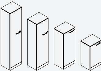
FS200 FS200-83: W 45 x D 36.6 x H 83 (L/R) FS200-120.5: W 45 x D 36.6 x H 120.5 (L/R) FS200-158: W 45 x D 36.6 x H 158 (L/R) FS200-195.5: W 45 x D 36.6 x H 195.5 (L/R) Capability of ordering mangnetic door
