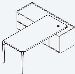
CM200 CM200-180: W 180 x D 90 x H 76 (Total Dim: 205x170x76) CM200-200: W 200 x D 90 x H 76 (Total Dim: 225x170x76) CM200-220: W 220 x D 90 x H 76 (Total Dim: 245x170x76) Sideboard: W 170 x D 60 x H 66
