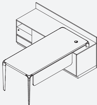
CM400 CM400-180: W 180 x D 90 x H 76 (Total Dim: 205x180x76) CM400-200: W 200 x D 90 x H 76 (Total Dim: 225x180x76) CM400-220: W 220 x D 90 x H 76 (Total Dim: 245x180x76) Sideboard: W 180 x D 60 x H 70
