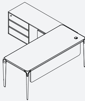
CD100 CD100-150: W 150 x D 75 x H 76 (Total Dim: 162x197x76) CD100-160: W 160 x D 75 x H 76 (Total Dim: 172x197x76) CD100-180: W 180 x D 75 x H 76 (Total Dim: 192x197x76) Sideboard: W 160 x D 50 x H 64
