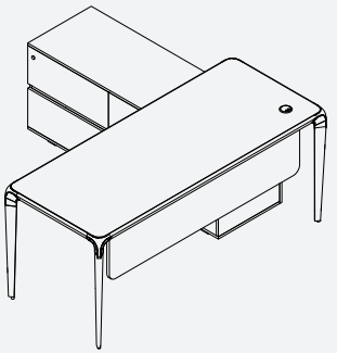
CD200 CD200-150: W 150 x D 75 x H 76 CD200-160: W 160 x D 75 x H 76 CD200-180: W 180 x D 75 x H 76 Sideboard: W 150 x D 50 x H 64
