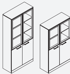
FS450 FS450-158: W 90 x D 36.6 x H 158 FS450-195.5: W 90 x D 36.6 x H 195.5 Capability of ordering mangnetic door
