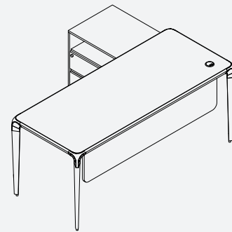
CD300 CD300-150: W 150 x D 75 x H 76 (Total Dim: 150x136x76) CD300-160: W 160 x D 75 x H 76 (Total Dim: 160x136x76) CD300-180: W 180 x D 75 x H 76 (Total Dim: 180x136x76) Sideboard: W 90 x D 50 x H 64
