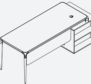
CD400 CD400-140: W 140 x D 75 x H 76 (Total Dim: 160x75x76) CD400-150: W 150 x D 75 x H 76 (Total Dim: 170x75x76) CD400-160: W 160 x D 75 x H 76 (Total Dim: 180x75x76) CD400-180: W 180 x D 75 x H 76 (Total Dim: 200x75x76) Sideboard: W 63 x D 75 x H 64
