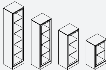
FS500 FS500-83: W 45 x D 36.6 x H 83 (L/R) FS500-120.5: W 45 x D 36.6 x H 120.5 (L/R) FS500-158: W 45 x D 36.6 x H 158 (L/R) FS500-195.5: W 45 x D 36.6 x H 195.5 (L/R) Capability of ordering mangnetic door
