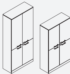
FS350 FS350-158: W 90 x D 36.6 x H 158 FS350-195.5: W 90 x D 36.6 x H 195.5 Capability of ordering mangnetic door
