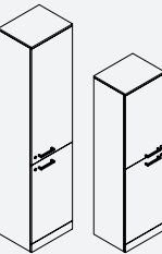
FS300 FS300-158: W 45 x D 36.6 x H 158 (L/R) FS300-195.5: W 45 x D 36.6 x H 195.5 (L/R) Capability of ordering mangnetic door
