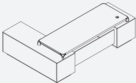
CM100 CM100-200: W 200 x D 90 x H 76 (Total Dim: 240x180x76) CM100-220: W 220 x D 90 x H 76 (Total Dim: 260x180x76) Sideboard 1: W 180 x D 60 x H 64 Sideboard 2: W 95 x D 60 x H 64
