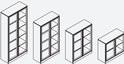
FS550 FS550-83: W 90 x D 36.6 x H 83 FS550-120.5: W 90 x D 36.6 x H 120.5 FS550-158: W 90 x D 36.6 x H 158 FS550-195.5: W 90 x D 36.6 x H 195.5 Capability of ordering mangnetic door
