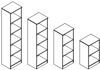
FS100 FS100-83: W 45 x D 36.6 x H 83 FS100-120.5: W 45 x D 36.6 x H 120.5 FS100-158: W 45 x D 36.6 x H 158 FS100-195.5: W 45 x D 36.6 x H 195.5
