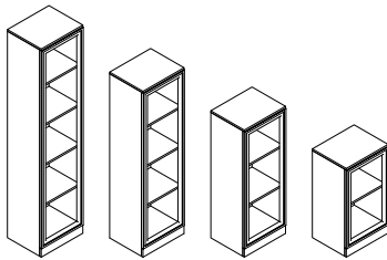
FS500 FS500-83: W 45 x D 36.6 x H 83 ( R / L ) FS500-120.5: W 45 x D 36.6 x H 120.5 ( R / L ) FS500-158: W 45 x D 36.6 x H 158 ( R / L ) FS500-195.5: W 45 x D 36.6 x H 195.5 ( R / L ) Capability of ordering magnetic door
