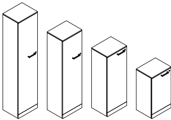
FS200 FS200-83: W 45 x D 36.6 x H 83 ( L / R ) FS200-120.5: W 45 x D 36.6 x H 120.5 ( L / R ) FS200-158: W 45 x D 36.6 x H 158 ( L / R ) FS200-195.5: W 45 x D 36.6 x H 195.5 ( L / R ) Capability of ordering magnetic door
