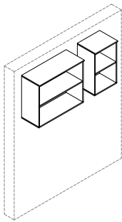
FL200 FL200-45: W 45 x D 36.6 x H 75 FL200-90 : W 90 x D 36.6 x H 75
