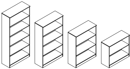
FS150 FS150-83: W 90x D 36.6 x H 83 FS150-120.5: W 90 x D 36.6 x H 120.5 FS150-158: W 90 x D 36.6 x H 158 FS150-195.5: W 90 x D 36.6 x H 195.5
