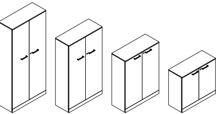
FS250 FS250-83: W 90x D 36.6 x H 83 FS250-120.5: W 90 x D 36.6 x H 120.5 FS250-158: W 90 x D 36.6 x H 158 FS250-195.5: W 90 x D 36.6 x H 195.5 Capability of ordering magnetic door
