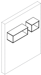
FL100 FL100-45 : W 45 x D 36.6 x H 37.5 FL100-90 : W 90 x D 36.6 x H 37.5
