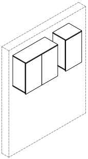
FL400 FL400-45 : W 45 x D 36.6 x H 75 FL400-90 : W 90 x D 36.6 x H 75
