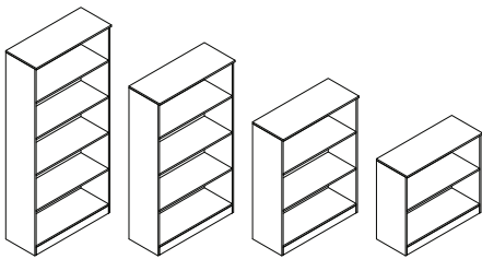
FS150 FS150-83: W 90x D 36.6 x H 83 FS150-120.5: W 90 x D 36.6 x H 120.5 FS150-158: W 90 x D 36.6 x H 158 FS150-195.5: W 90 x D 36.6 x H 195.5
