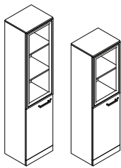
FS400 FS400-158: W 45 x D 36.6 x H 158 ( R / L ) FS400-195.5 W 45 x D 36.6 x H 195.5 ( R / L ) Capability of ordering magnetic door
