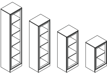
FS500 FS500-83: W 45 x D 36.6 x H 83 (R / L ) FS500-120.5: W 45 x D 36.6 x H 120.5 (R / L ) FS500-158: W 45 x D 36.6 x H 158 (R / L ) FS500-195.5: W 45 x D 36.6 x H 195.5 (R / L ) Capability of ordering magnetic door
