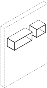
FL100 FL100-45 : W 45 x D 36.6 x H 37.5 FL100-90 : W 90 x D 36.6 x H 37.5
